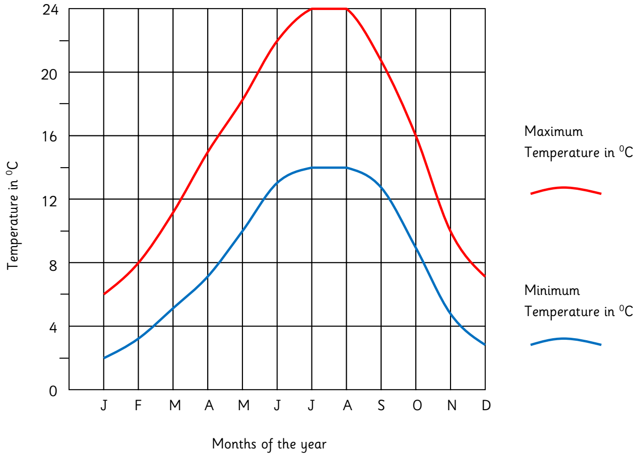
Average monthly maximum and minimum temperatures in Paris
